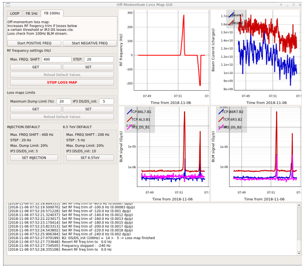
Figure 3: Graphical user interface for the beam loss off-momentum feedback.
