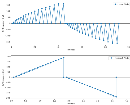
Figure 2: Simulated RF frequency change over time for the Loop Mode (top) and for the Feedback Mode (bottom).
