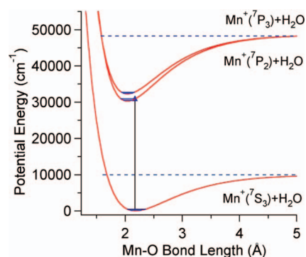
FIG. 3. Potential energy curves of the ground and excited electronic states of \text{Mn}^+(\text{H}_2\text{O}) along the \text{Mn}-\text{O} stretch based on experiment.
