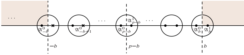
Figure 2. The complex \mathcal{C} after contraction when p > 0 .
