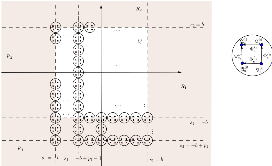
Figure 7. Truncated complex for p_1 > 0, p_2 < 0 .
