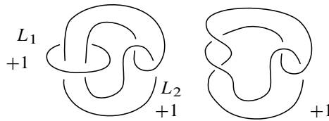
Figure 12. After +1 surgery along component L_1 of the positively-clasped Whitehead link we obtain the right-handed trefoil in S^3 .
