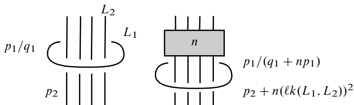
Figure 11. A Rolfsen twist. Here we take p_1/q_1 = \pm 1 and n = \mp 1 .
