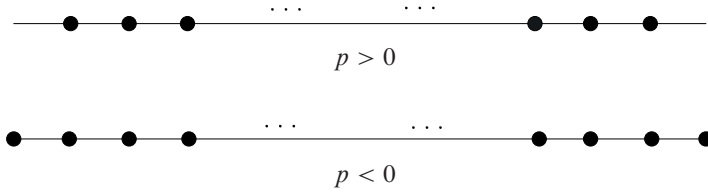
Figure 4. The complex CW(p, i, b) .
