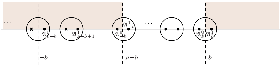
Figure 3. The complex \mathcal{C} after contraction when p < 0 .
