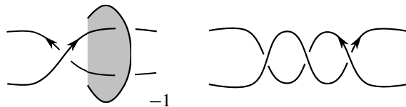
Figure 13. A crossing change taking D_+ to D_- .
