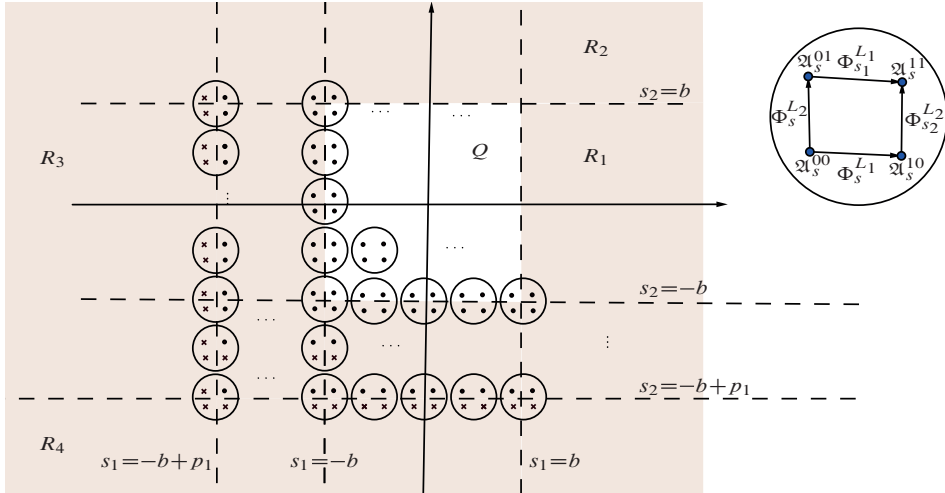
Figure 6. Truncated complex for p_1, p_2 < 0
