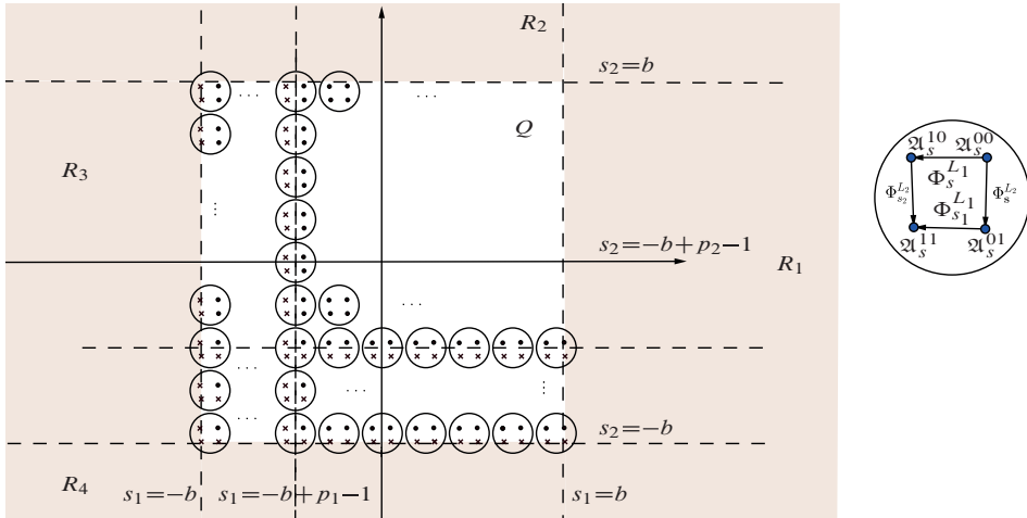
Figure 5. Truncated complex for p_1, p_2 > 0 .
