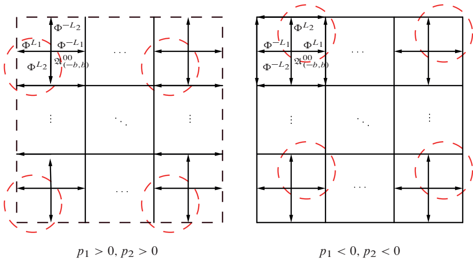
Figure 8. Cases (a) and (b).
