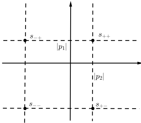
Figure 10. For each \text{Spin}^c -structure i , there is a unique point s_{\pm\pm}(i) in each quadrant that is the closest to the origin.
