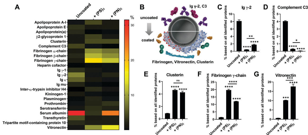
Fig. 2 Comparison of adsorbed proteins between uncoated liposomes and lipo-dendrimers (lipo-(PS) 4 and lipo-(PN) 8 ) in human plasma. (A) Heatmap of adsorbed proteins to lipo-(PS) 4 and lipo-(PN) 8 in human plasma. Each protein amount is given in % relative to the total amount of all identified proteins. A list of all identified proteins is provided in Table S1 (ESI † ). (B) Coating of liposomes lead to a different protein corona: reduction of (C) Ig \gamma -2 adsorption and (D) complement C3 and enhancement of (E) clusterin, (F) fibrinogen and (G) vitronectin ( n = minimum 2; one-way ANOVA; not significant (ns) for p > 0.05 , * for p \leq 0.05 , ** for p \leq 0.01 , *** for p \leq 0.001 , **** for p \leq 0.0001 ).
