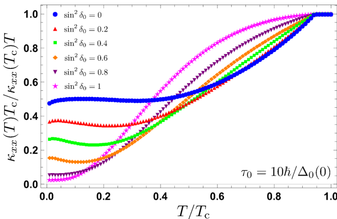
FIG. 5. Temperature dependence of the longitudinal thermal conductivity divided by temperature \kappa_{xx}/T normalized by the value at the transition temperature without impurities and external fields T_c for the different scattering phase shifts \sin^2 \delta_0 = 0, 0.2, \dots, 1 at the relaxation time \tau_0 = 10\hbar/\Delta_0(0) .
