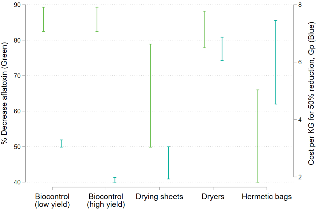
Figure 3: Efficacy and cost-effectiveness of technologies for aflatoxin control in crops
