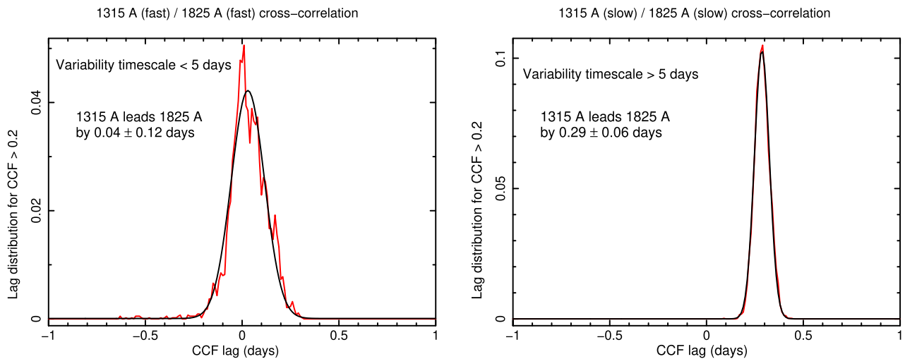
Figure 6. The effect of light-curve filtering in UV: Left-hand panel shows relative frequency distribution of CCFs computed with 1315 and 1825 Å UV continuum light curves (left-hand panel of Fig. 5) after applying a slow filter that only preserves fast (faster than 5 d) variability. On the other hand, when a fast filter is applied that only preserves slow (slower than 5 d) variability, the resulting CCF is shown in the right-hand panel. Both distributions are fitted with a Gaussian whose centroid and FWHM/2 are quoted as the time delay and its uncertainty, respectively. A significant difference between the fast and slow variability delay measurements can be noted.
