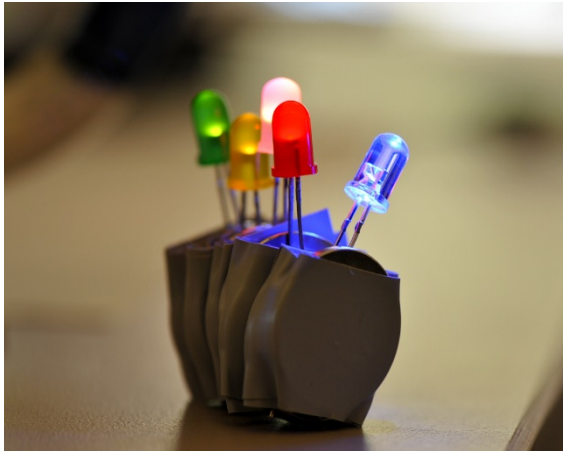
Figure 4-7 LED throwies.
