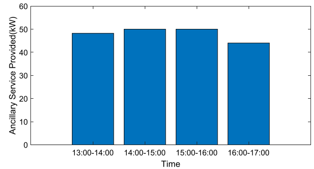
Fig. 11. The total amount of ancillary service provided by the community for 13:00–17:00 in Case 3.
