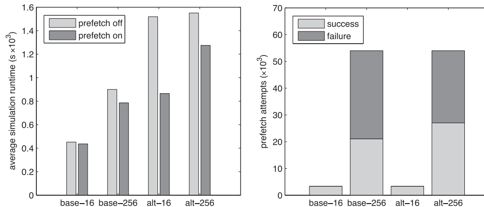
Fig. 9. Prefetching results.
