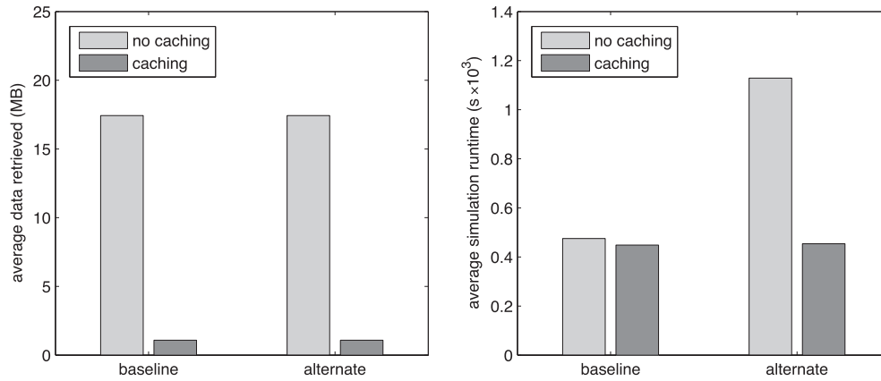
Fig. 8. Caching results.
