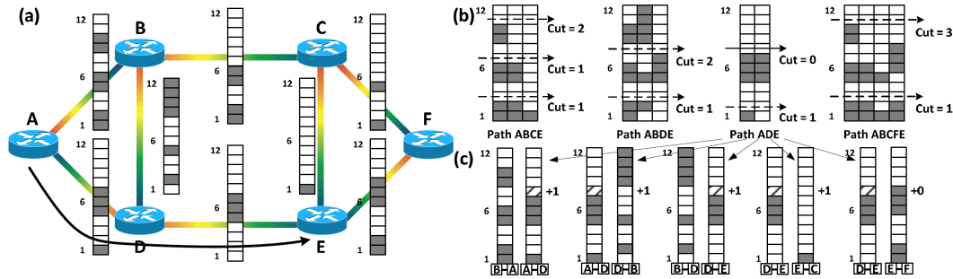
Figure 3.4: Example FISH network and the spectral assignment status on the links, (b) number of cuts to all the candidate solution to connection request A-E, and (c) alignment factor increase if choosing path ADE with slot 8 [4]
