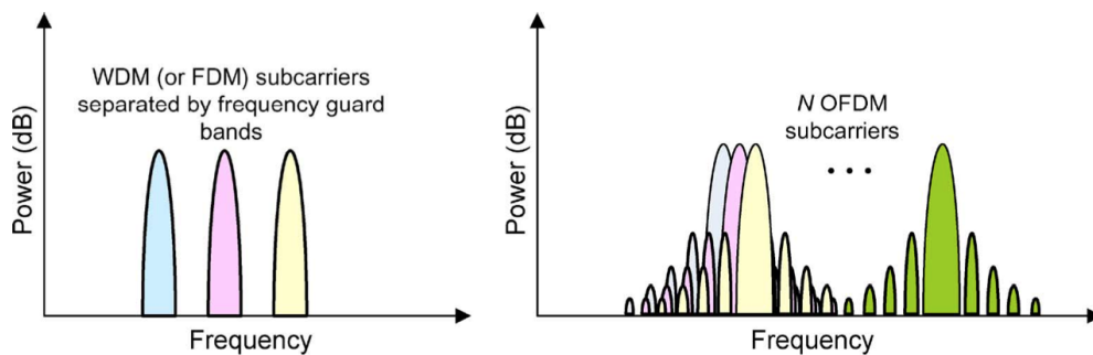
Figure 2.3: Spectrum of (a) WDM or FDM signals (b) OFDM signal [1]
