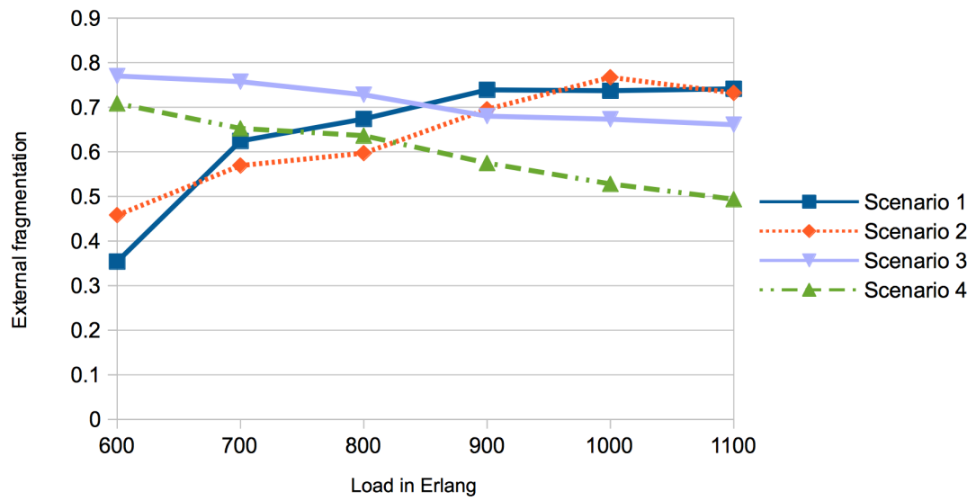
Figure 7.13: Spectrum fragmentation level in Nobel German network topology
