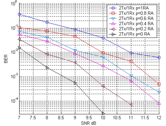
Fig. 10. BER performance of DVB-H with CDD-2Tx in correlated RA.
