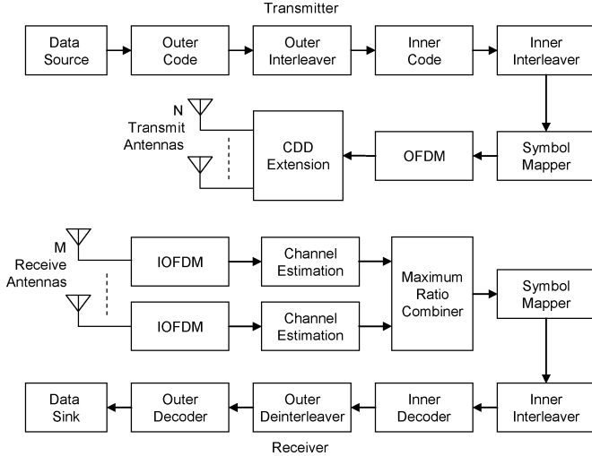
Fig. 1. System model of DVB-H with CDD extension.
