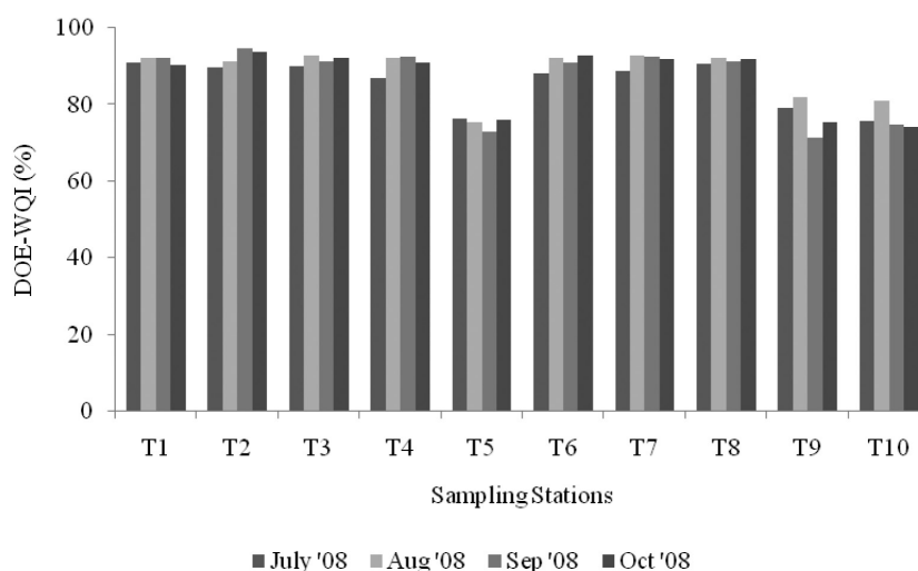
FIGURE 3. Variation of the DOE-WQI for the different sampling stations
