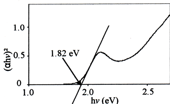
FIGURE 2. Plotting of (ahv)^2 versus hv for optical energy band gap calculation for QDs core grown for 10 minutes
