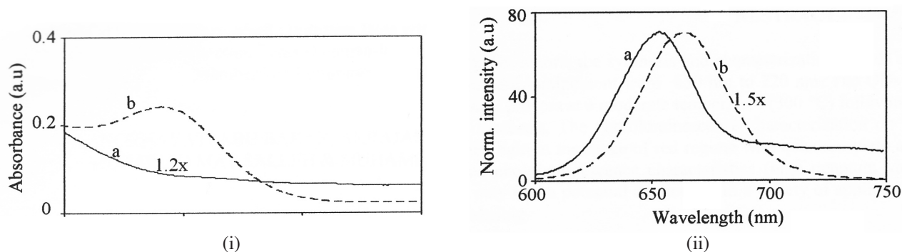
FIGURE 4. These spectra a) CdTe-CdSe core-shell b) CdTe-core QDs for graphs: i) the UV-Vis absorption spectra and, ii) the corresponding photoluminescence spectra
