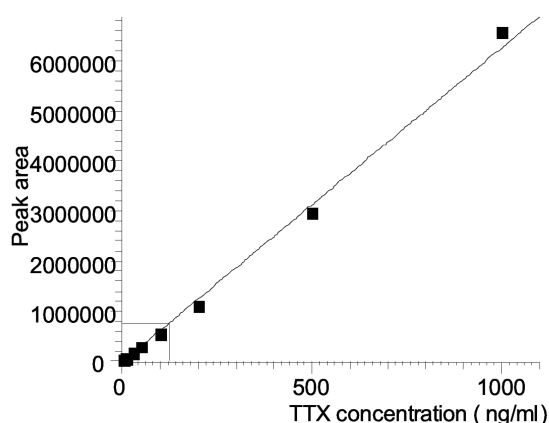
FIGURE 2. Calibration curves of TTX obtained by LC-MS/MS
