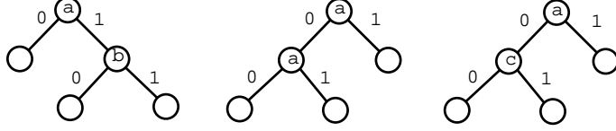
Fig. 5. Adaptive test cases \gamma_1 , \gamma_2 , and \gamma_3
