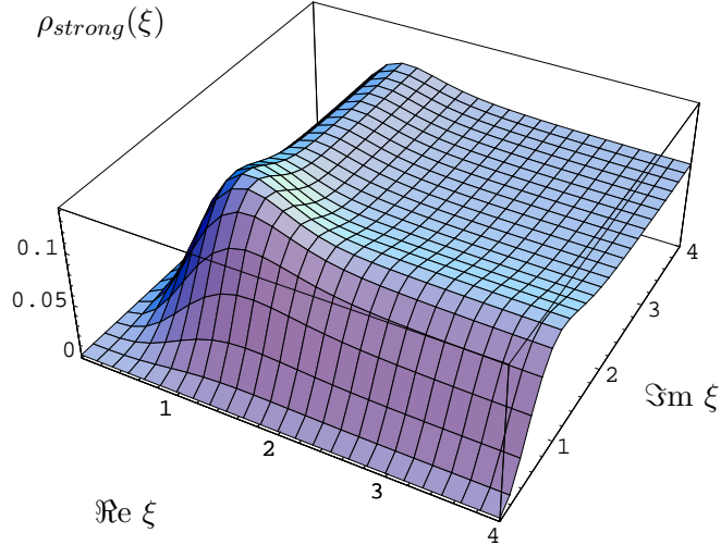
Figure 8: Part of Fig. 7 (left) showing the first quadrant only. The symmetry with respect to the diagonal \Re\xi = \Im\xi is clearly visible .
