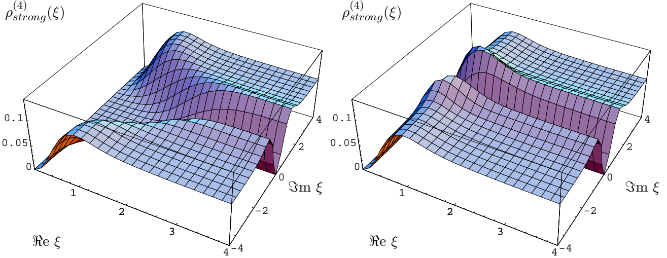
Figure 10: The massive spectral density at mass \eta = 0.5 (left) and \eta = 8 (right), both with \nu = 0 .
