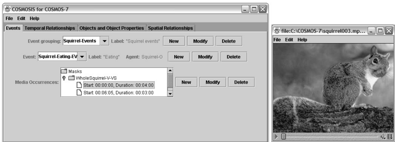
Fig. 5: COSMOSIS.
