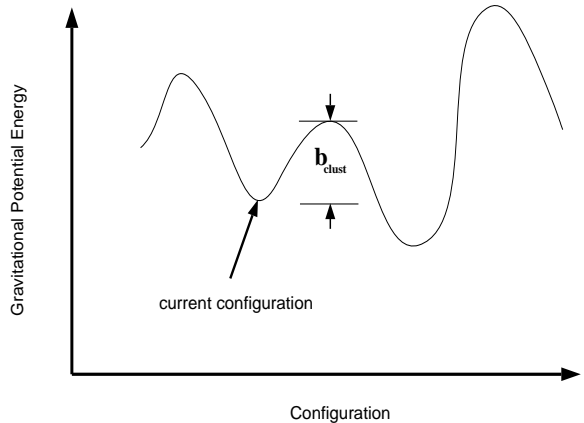
FIG. 2. Schematic example of a potential energy landscape for an ensemble of granules in configuration space. The ensemble currently lies at the local minimum marked. The smallest barrier to an adjacent minimum has a height of b_{\text{clust}} .
