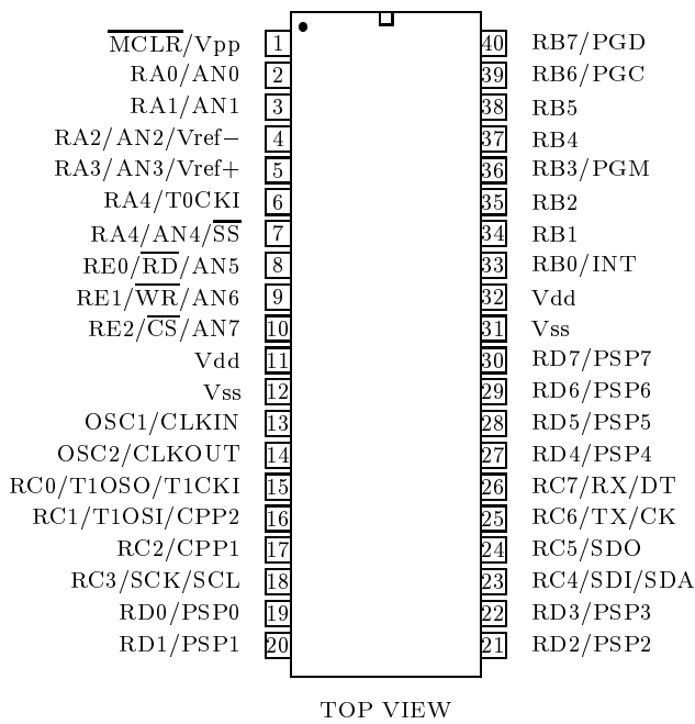
(f) PIC 16F877
