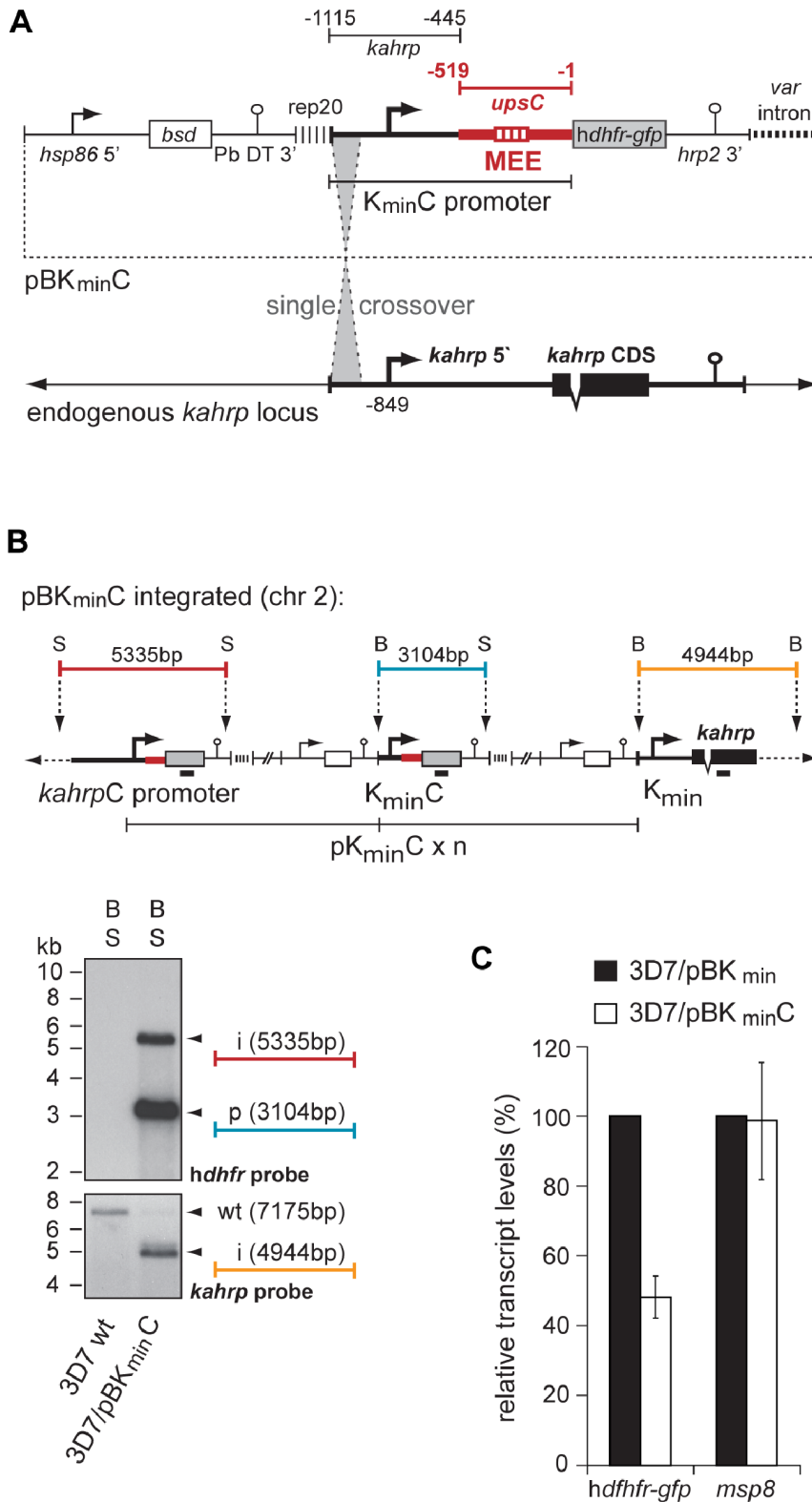
Figure 1. Integration of the upsC 5' upstream sequence into a heterologous context at the kahrp locus. (A) Schematic map of the transfection construct pBK min C. Single-crossover integration was guided by kahrp 5' homology. The position of the kahrp TSS is indicated [81]. Numbers refer to the nucleotide positions relative to the ATG start codon. The bsd resistance cassette selects for stably transfected parasites. The var intron is indicated by a bold dashed line. hsp86 5', hsp86 promoter; Pb DT 3', P. berghei dhfr -thymidylate synthase terminator; rep20, 0.5 kb TARE6 repeat element; hrp2 3'; histidine-rich protein 2 terminator. MEE, location of the 101 bp mutual exclusion element MEE [54]. (B) Genomic situation after integration of the pBK min C concatamer into the endogenous kahrp locus. Restriction sites used in Southern analysis and fragment lengths are indicated and colour-coded. S, Stul ; B, BglII . The Southern blot on BglII/Stul -digested gDNA shows integration of pBK min C into the endogenous locus
