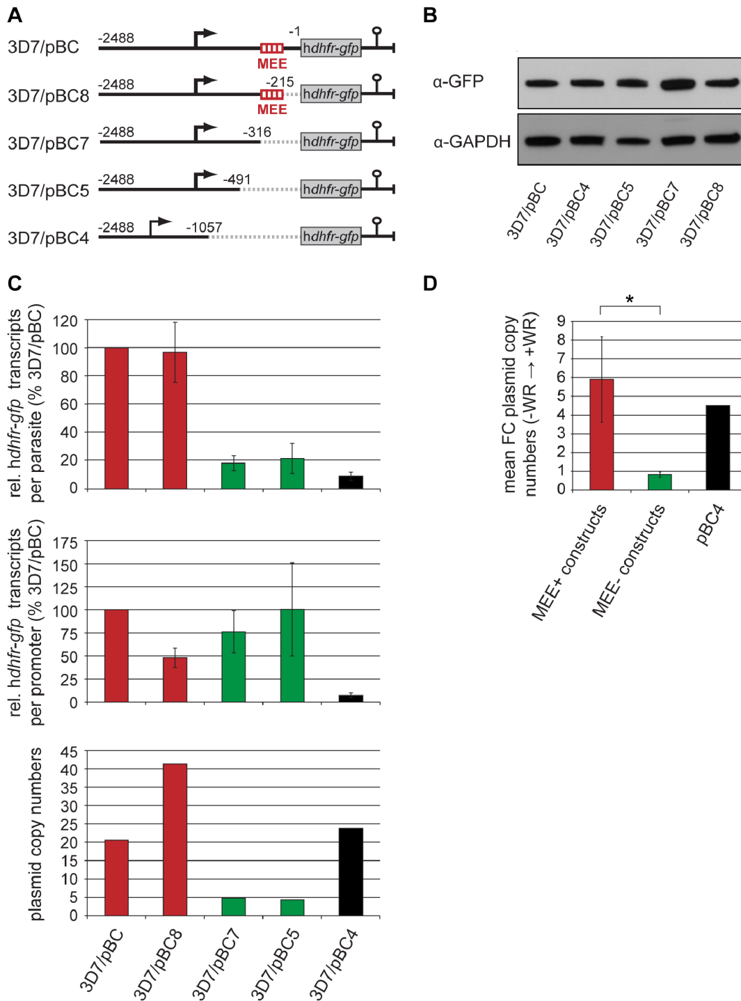
Figure 4. The MEE inhibits translation in the natural context of the upsC promoter. (A) Schematic depiction of upsC var promoter reporter constructs [54]. Deletions are represented by dashed lines. Numbers refer to the nucleotide positions relative to the ATG start codon. The position of the MEE is highlighted. (B) Expression of hDHFR-GFP and GAPDH (loading control) in WR-selected parasites was analysed by semi-quantitative Western blot. (C) Top panel: Proportion of total steady-state hdhfr-gfp transcripts in WR-selected parasites carrying truncated upstream sequences relative to the control line 3D7/pBC. Values are derived from three independent experiments (mean \pm s.d.) (normalised to PF3D7_1331700 transcripts). Middle panel: Proportion of steady-state hdhfr-gfp transcripts produced by a single promoter in WR-selected parasites carrying truncated upstream sequences relative to the control line 3D7/pBC. Values represent the data displayed in the top panel divided by the average plasmid copy number determined from the same batch of parasites (bottom panel). (D) Mean increase in plasmid copy numbers ( \pm s.d.) after WR selection in parasites transfected with constructs carrying MEE-positive upstream sequences (red) or MEE-negative upstream sequences (green). The increase in plasmid copy numbers in WR-selected 3D7/pBC4 is shown in black. Individual plasmid copy numbers determined for each population are shown in Figure S3. Asterisk, p=0.0015 (Student's t-test). doi:10.1371/journal.pone.0100183.g004
