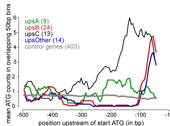
Figure 5. uAUGs are enriched in var 5' UTRs. For each gene, sequences ranging from bp -500 to -1 relative to the ATG start codon were downloaded from PlasmoDB version 7.2 ( www.plasmoDB.org ) and the counts of the trinucleotide sequence 'ATG' were assessed in sliding windows of 50 bps using custom-made Perl scripts. The average ATG counts for each sequence set were plotted using the statistical analysis package R ( www.r-project.org ). The var gene set includes 60 sequences, subdivided into groups "upsA", "upsB", "upsC" and "others" ( upsB/C , upsB/A , upsE ) according to the classification by Lavstsen and colleagues [15]. The control set consists of 5' UTR sequences of 403 genes with peak transcription in ring stages. Selection of these sequences was based on RNASeq data [39] according to the following criteria: timing of maximal expression: 8 hpi and 16 hpi; maximal expression ratio: 8-fold induction; maximum expression percentile: 30 th percentile. uAUGs are significantly enriched in var 5' UTRs compared to the control set of ring stage-specific genes ( p = 7.56 \times 10^{-11} ; Welch t-test). doi:10.1371/journal.pone.0100183.g005
