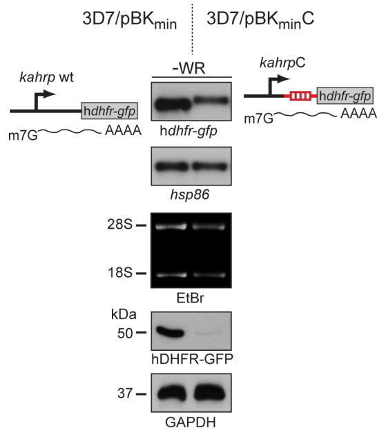
Figure 2. The upsC 5' UTR element inhibits translation. Semi-quantitative analysis of transcript and protein abundance in 3D7/pBK min (control) and 3D7/pBK min C ring stage parasites (6–14 hpi) cultured in absence of WR (−WR). Top panels: hdhfr-gfp and hsp86 (loading control) transcripts were detected by Northern blot. Ethidium bromide-stained 18S and 28S rRNAs serve as second loading control. Bottom panels: expression of hDHFR-GFP and GAPDH (loading control) in the same parasite samples were analysed by Western blot. doi:10.1371/journal.pone.0100183.g002
