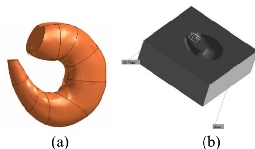
Figure 6. (a) The finished 3D model of shelled shrimp; (b) The finished cavity plate of shelled shrimp.
