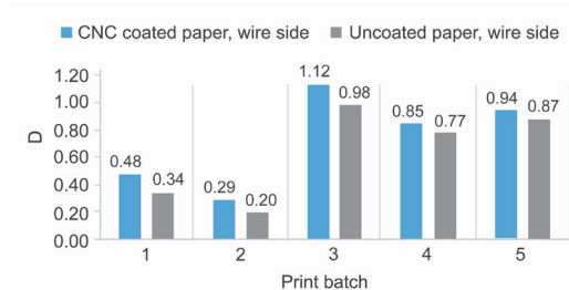
Figure 4 Density of set-off prints with 3 s interval, two fields; 1 - Set-off paper, 1st contact; 2 - Set-off paper, 3 s interval; 3 - Test paper, printed only; 4 - Test paper, 1st contact; 5 - Test paper, 3 s interval CNC coated paper, wire side and uncoated
