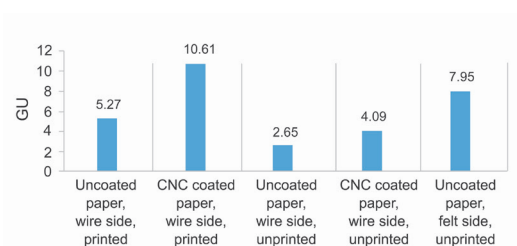
Figure 2 Surface and print gloss of unprinted and printed CNC coated and uncoated paper samples
