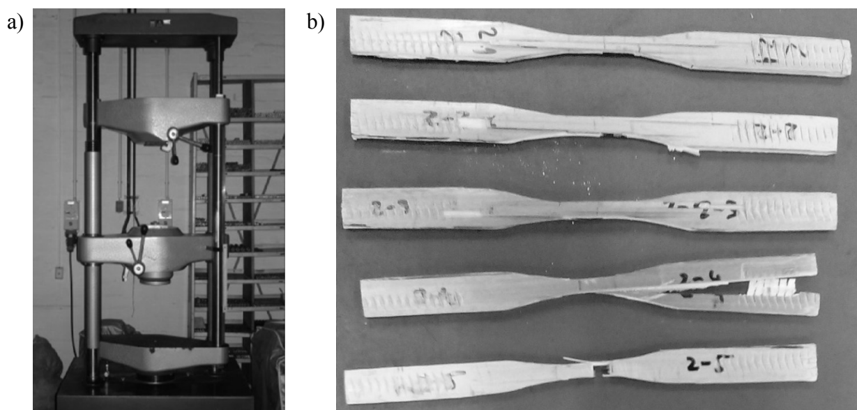
Figure 3. a) Test machine b) tested samples.
