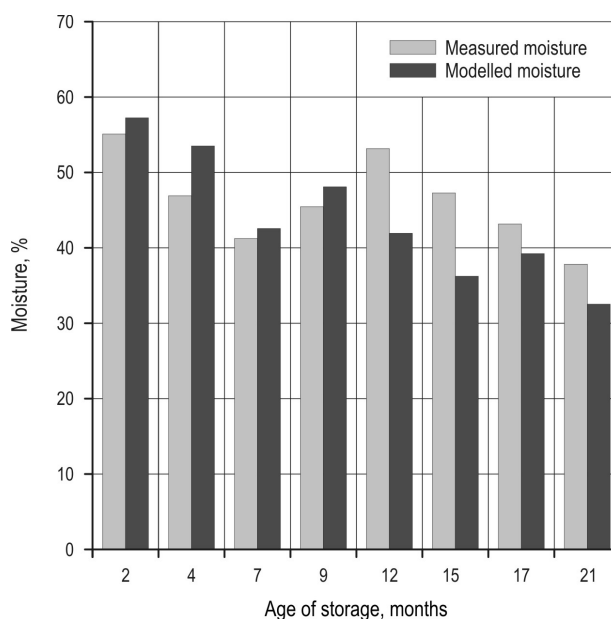
Fig. 6 Measured and modelled moisture content of 8 different uncovered energy wood piles
