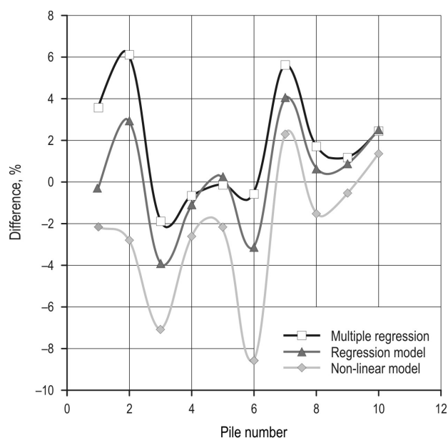
Fig. 4 Difference between measured and modelled moisture with different model types, pine stem wood, covered
