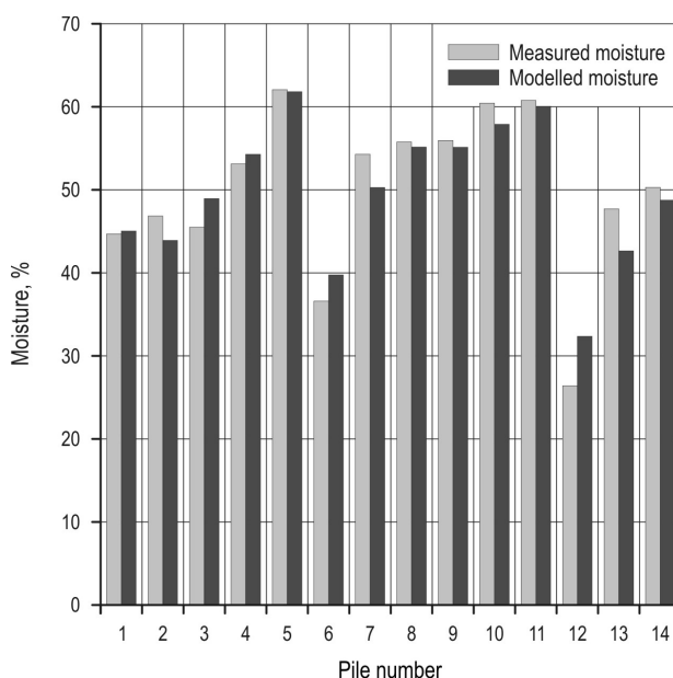
Fig. 5 Measured and modelled moisture content of 14 different covered energy wood piles
