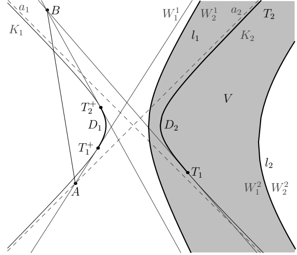
Figure 7: For the component K_1 , the set of exterior points of contact D_{ext}^1 = \emptyset and the set of interior points of contact D_{in}^1 = \widehat{T_1^+ T_2^+} . The set of points of contact D^1 = D_{in}^1 generates the curve l_1 \subset \partial V_\rho(A, B) . The curve l_1 divides the plane \rho into two regions W_1^1, W_2^1 . Let the points A, B \in W_1^1 . According to the theorem 7, the set of admissible solutions for the component K_1 is V^1(A, B) = W_2^1 .
