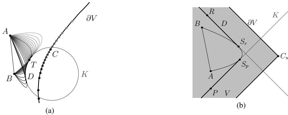
Figure 5: (a) The boundary map \sigma maps the points of the arc D to the points on \partial V , see that \sigma(T) = C . (b) Let the conic section K = p \cup r . The points A, B have to lie in the same quadrant with respect to K . Let the quadrant be determined by two half-lines \overrightarrow{V_Q P} \subset p and \overrightarrow{V_Q R} \subset r . If there exists a Bézier curve b_{AC_u B} with double contact M = \{S_p, S_r\} with K , the set of exterior points of contact D_{ext} = \overrightarrow{S_p P} \cup \overrightarrow{S_r R} . Otherwise, we get S_p = S_r = V_Q and D_{ext} = \overrightarrow{V_Q P} \cup \overrightarrow{V_Q R} . The set of interior points of contact is always D_{in} = \emptyset . The boundaries generated by the half-lines \overrightarrow{S_p P}, \overrightarrow{S_r R} are connected due to the fact that \sigma(S_p) = \sigma(S_r) = C_u . Hence, the set of admissible solution V_\rho(A, B) consist of one region. Because the boundary is generated by the exterior points of contact, A, B \in V_\rho(A, B) .
