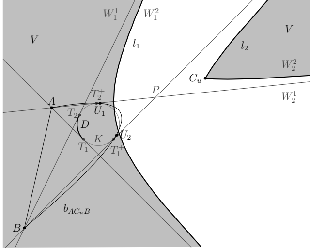
Figure 4: The set D_{ext} = \{X \in K: A\vec{Q}_K X^\top > 0 \wedge B\vec{Q}_K X^\top > 0\} = \widehat{T_1 T_2} . The set D_{in} \neq \emptyset , because the point P lies in the same half-plane generated by \overleftrightarrow{AB} as the points T_1^+, T_2^+ . The set D_{in} = \{X \in K: A\vec{Q}_K X^\top < 0 \wedge B\vec{Q}_K X^\top < 0\} \setminus \{U_1 U_2\} consists of two affiliated components T_2^+ U_1 \cup U_2 T_1^+ \cup \{U_1, U_2\} . The split of the arc is caused by the existence of the curve b_{AC_uB} , which has double contact with the conic section K . As one can see, b_{AC_uB} \cap K = \{U_1, U_2\} . Therefore, the set of points of contact D = D_{ext} \cup D_{in} generates the curves l_1, l_2 such that l_1 \cup l_2 = \partial V_\rho(A, B) . Because the curve l_1 is generated by the exterior points of contact, the region W_1^1 containing the points A, B is subset W_1^1 \subset V_\rho(A, B) . The curve l_2 is generated by the interior points of contact. It bounds region W_2^2 not containing the points A, B and W_2^2 \subset V_\rho(A, B) according to theorem 7. The set of admissible solutions V_\rho(A, B) = W_1^1 \cup W_2^2 consists of two regions.
