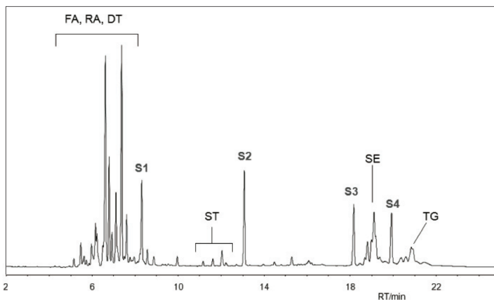
Figure 2 GC-FID (short column) chromatogram of heartwood hexane extract (tree 1 – 0.5 m stem height) (FA – fatty acids, RA – resin acids, DT – diterpenoids, ST – sterols, SE – sterol esters, TG – triglycerides, S1-S4 – internal standards)
