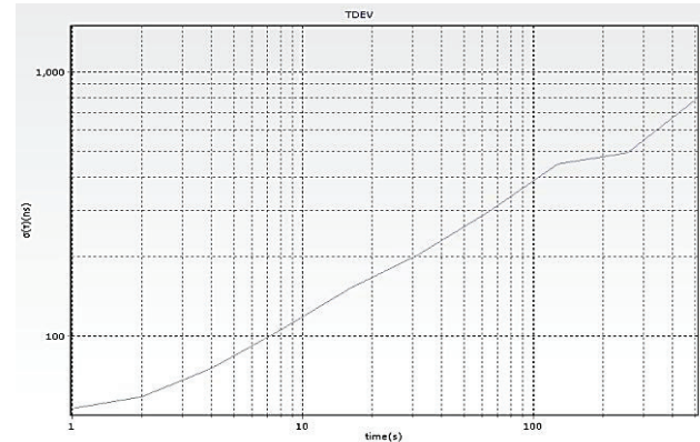
Figure 12 TDEV
