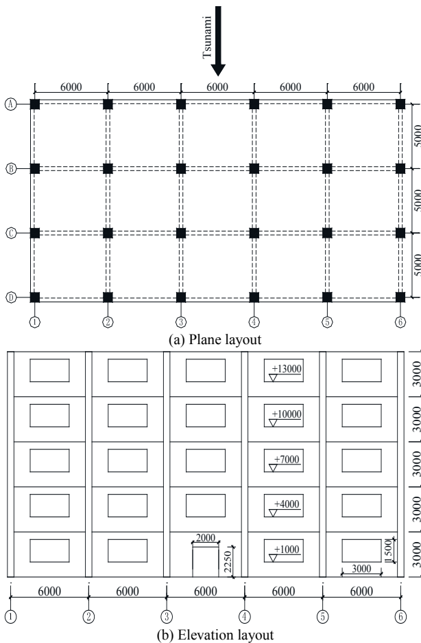
Figure 1 Plane and elevation layout of the structure (in mm)
