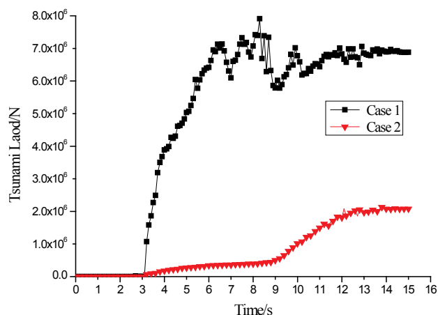
Figure 4 Time-history curves of tsunami wave horizontal thrust
