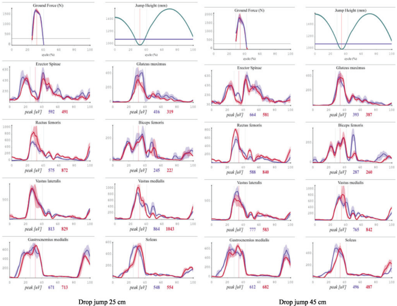
Fig. 5. EMG activation of muscles of lower extremities in the 25 and 45 cm drop jump.
