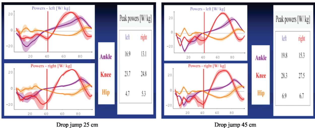
Fig. 3. Joint strength (P) in hips, knees and ankles, normalised to body mass (Wkg-1) according to Vaughan et al., 1999.
