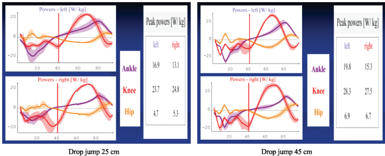
Fig. 2. Bilateral ground reaction force (L, R) in 25 and 45 cm drop jumps
