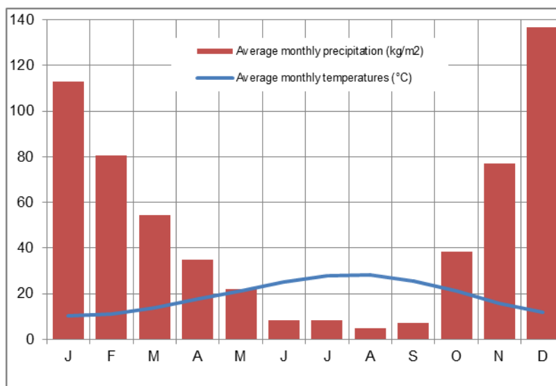
Figure 2. Climatogram of province Mersin from southern Turkey. (Turkish State Meteorological Service, 2015) Slika 2. Klimatogram provincije Mersin iz južne Turske. (Turkish State Meteorological Service, 2015)
