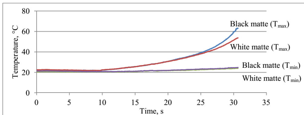
Slika 3. Izmjerene promjene temperature kod crnog mat i bijelog mat premaza Figure 3. The measured temperature changes with a black matte and white matte coating
