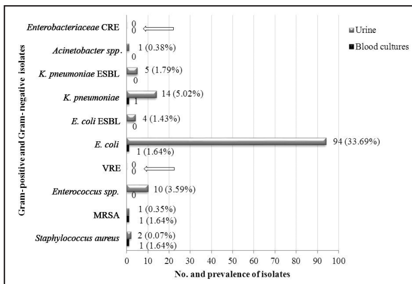
Figure 1. Gram-positive and Gram-negative bacteria isolated in blood and urine specimens and the prevalence of antimicrobial drugs' sensitive and multidrug-resistant strains.
