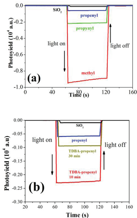
Figure 8. DC photo-yield vs. illumination time ( Y_{ph} vs. t ) collected at zero bias: (a) on \text{SiO}_2 and functionalized SiNWs/n-Si junction under 60 s white light illumination (AM 1.5, 100 \text{ mW cm}^{-2} ). (b) On RN propenyl-SiNWs/n-Si junction before and after further functionalization steps by TDBA molecules for 10(a) and 30 (b) minutes UV broadband lamp exposure (see ref 15, 16).
