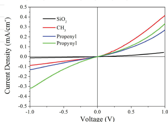
Figure 3. J vs V characteristics collected on RN of SiO 2 and molecularly functionalized SiNWs array on n-Si junction .
