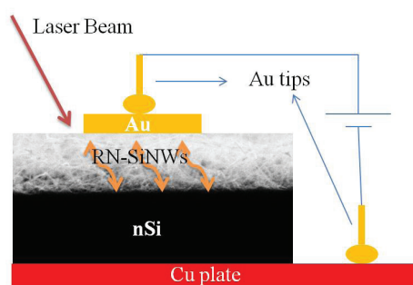
Figure 2. Schematic of the device configuration used for optoelectronic characterizations. A gold slab has been used instead of evaporated gold while InGa past has been painted on the back side of n-Si wafer for ohmic contact formation. The orange arrows is a simplified representation of the current percolation paths.
