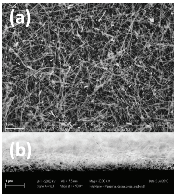
Figure 1. Typical top view and cross sectional SEM images of SiNWs random network on ( N_A \approx 10^{18}/\text{cm}^3 ) (111) n-Si substrates. SiNWs were prepared by the vapour-liquid-solid (VLS) method using chemical vapour deposition with silane and then terminated with different organic molecules using a chlorination/alkylation process (see ref.15 and 16)
