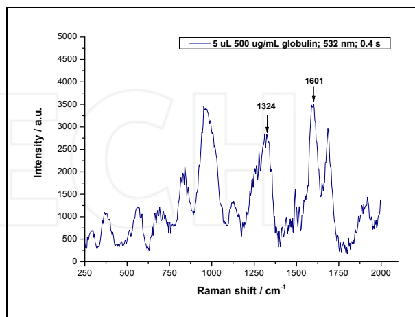
Figure 7. SERS spectrum of 5µL 500µg/mL globulin on a polished stainless steel target covered by Ag (CV scan number 25).
