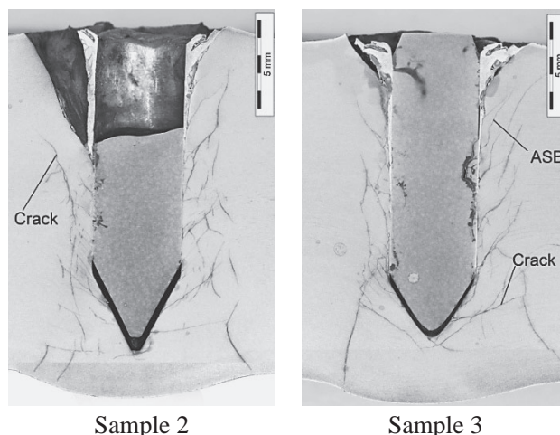
Figure 4 Macroscopic picture of breakthroughs bullets trough the samples 2 and 3, marked as cracks and ASB
