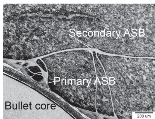
Figure 5 The microstructure of the cross-section of the target at the centre of the bullet. Course of ASB and cracks (sample 1)
