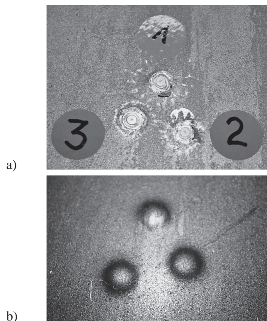
Figure 2 Front (a) and back (b) side of the steel plate PROTAC 500 after ballistic testing – details of three shots
