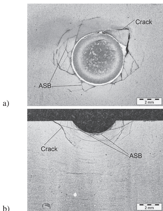
Figure 3 Macroscopic cross-sectional images of the sample 1 (a - upper level, b - lower level)
