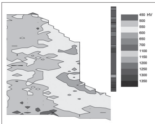
Figure 6 Distribution of hardness of the steel in the vicinity of the bullet penetration through sample 3
