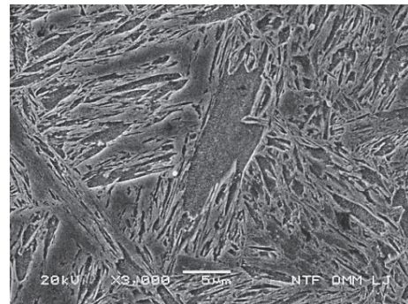
Figure 1 The microstructure of steel PROTAC 500 (SEM)
