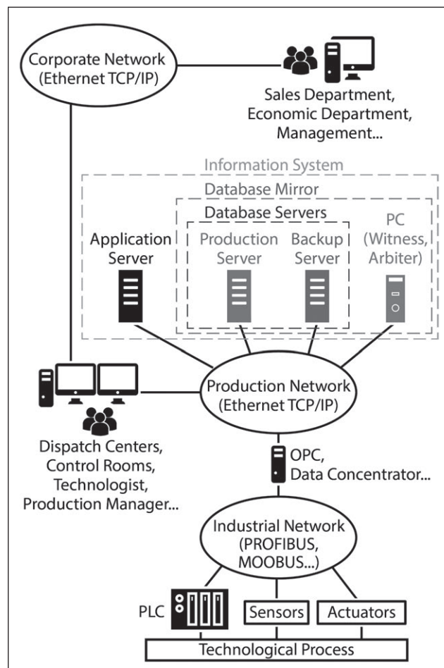
Figure 2 Model example of an information system for continuous process control. Source: own processing
