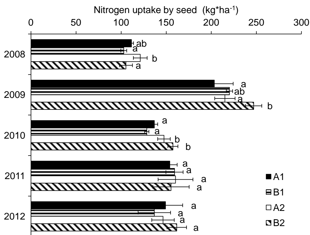
Figure 2. Effect of treatments on the nitrogen uptake by seed dry matter (kg*ha -1 ) during experimental years 2008-2012.
