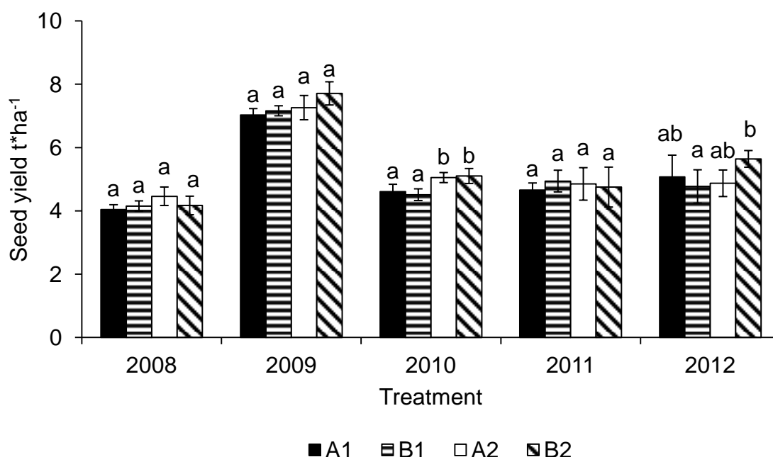
Figure 1. Seed yield ( \text{t}\cdot\text{ha}^{-1} ) at 12% moisture.
