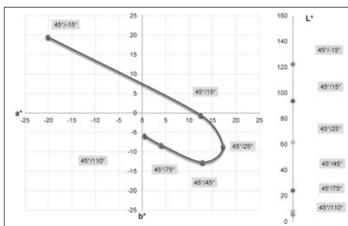
Figure 3. The CIEL*a*b* color coordinates of printed multi-color effect pigment applied on Foil 1, measured at various viewing angles.
