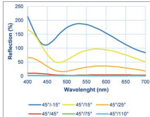
Figure 6. The reflection curves of printed multi-color effect pigment applied on black Foil 1, measured at various viewing angles.
