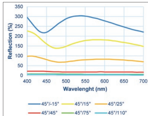
Figure 7. The reflection curves of printed multi-color effect pigment applied on Foil 2, measured at various viewing angles.
