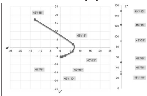
Figure 4. The CIEL*a*b* color coordinates of printed multi-color effect pigment applied on Foil 2, measured at various viewing angles.
