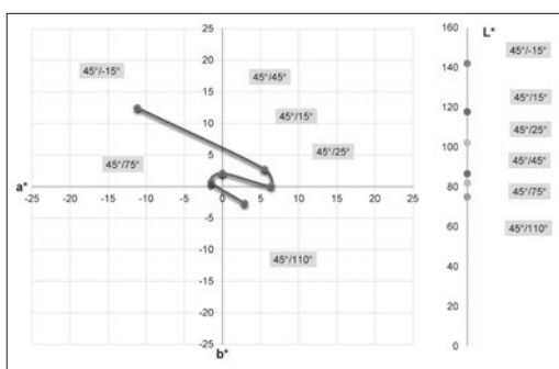
Figure 5. The CIEL*a*b* color coordinates of printed multi-color effect pigment applied on Foil 3, measured at various viewing angles.
