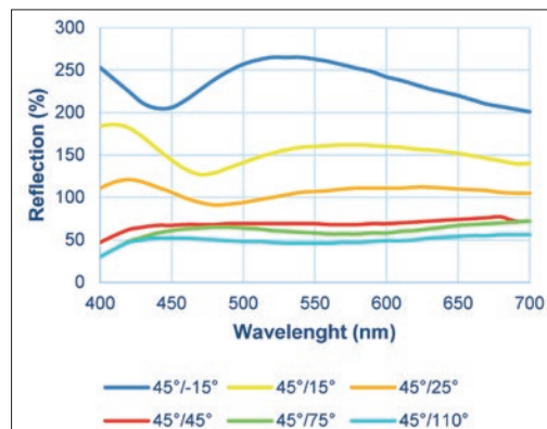
Figure 8. The reflection curves of printed multi-color effect pigment Foil 3, measured at various viewing angles.
