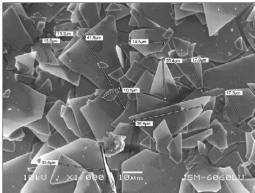
Figure 1. SEM image of multi-color effect pigment at 1000x magnification.
