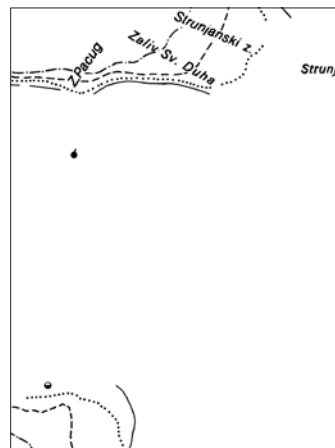
Figure 6. dark blue layer; the darker blue color marks sea, river, water area names which need to be visible inside the light blue of the water area (RGB 0, 175, 240)
