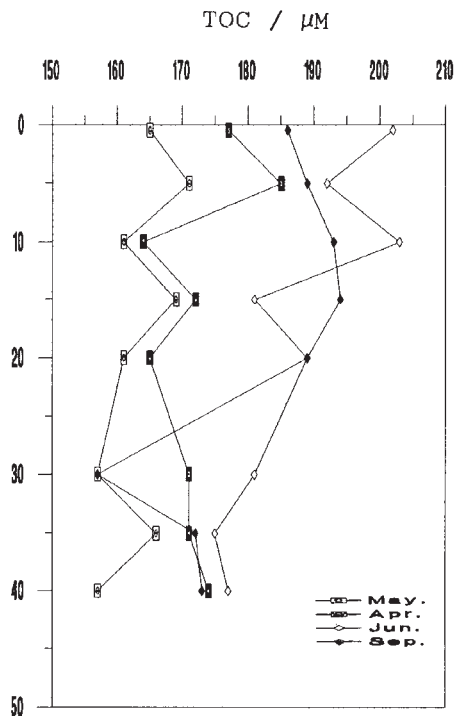
Figure 7. Total organic carbon profiles at station A.
