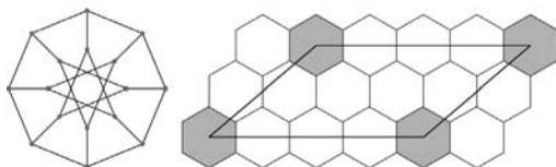
Figure 7. The Möbius-Kantor graph H(4,2,1) .
