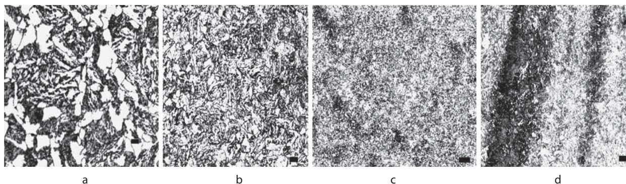
Figure 1 Structure of base material (AISI 4130): a – in case of plating by welding without ultrasonic activation; b – in case of plating by welding in ultrasonic field, in conditions: f = 33\ 867 / \text{Hz} , A = 38,9 / \mu\text{m} , I_s = 320 / A , v_s = 52,3 / \text{cm/min} ; c - in case of plating in ultrasonic field, in conditions: f = 38\ 204 / \text{Hz} , A = 62,7 / \mu\text{m} , I_s = 240 / A , v_s = 50,6 / \text{cm/min} ; d – in case of plating in ultrasonic field, in conditions: f = 35\ 797 / \text{Hz} , A = 70,5 / \mu\text{m} , I_s = 240 / A , v_s = 45,7 / \text{cm/min} ; zoom 200x
