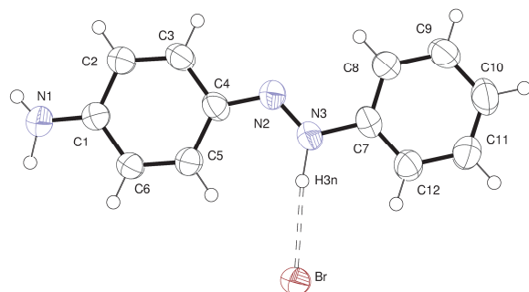
Figure 4. Figure 2 ORTEP III represented molecular structure of 2 .
