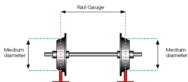
Figure 1 Axle assembly [1]
