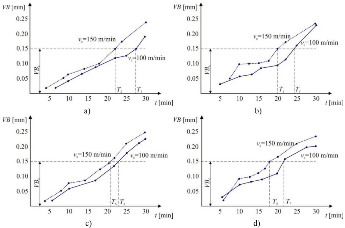
Figure 2 Wear profiles– down milling: a) f_t = 0,05 mm, a_e = 1 mm, (exp. 1 and 2), b) f_t = 0,11 mm, a_e = 1 mm, (exp. 3 and 4), c) f_t = 0,05 mm, a_e = 2 mm, (exp. 5 and 6), d) f_t = 0,11 mm, a_e = 2 mm, (exp. 7 and 8)
