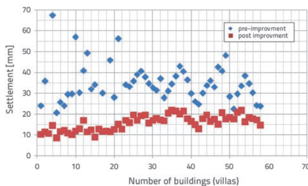
Figure 9. Settlement values based on the pre and post improvement CPTs
