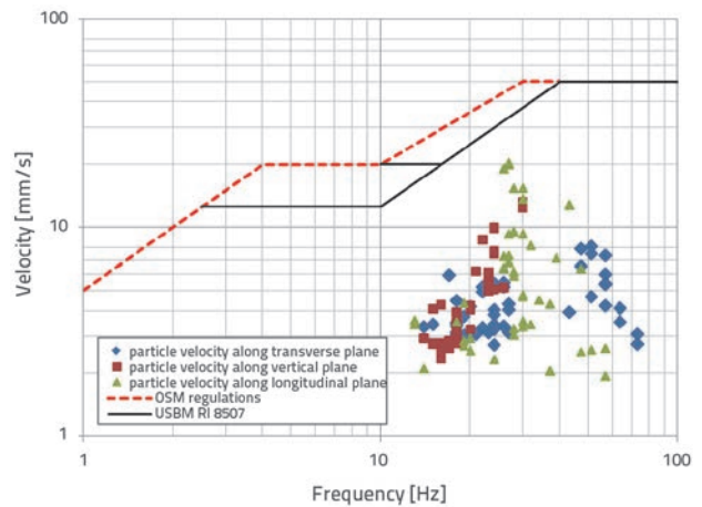
Figure 8. Vibration monitoring compared to the USBM RI8507 standards
