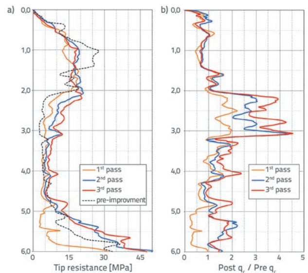
Figure 6. a) tip resistance for the pre-improvement, post 1 st , 2 nd , and 3 rd pass; b) post and pre improvement ratio q_c
