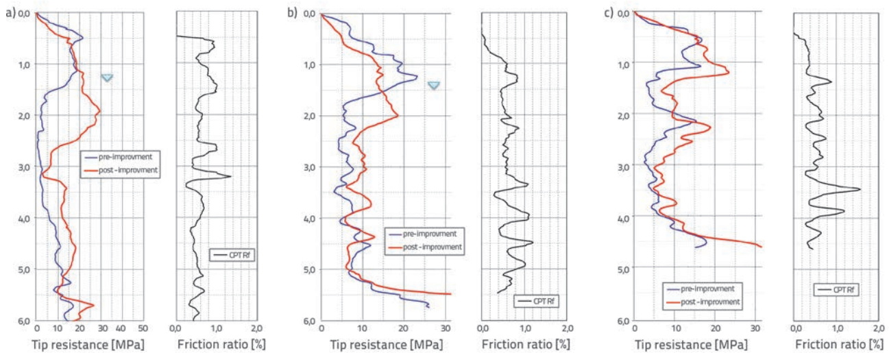
Figure 7. Pre and post improvement tip resistance
