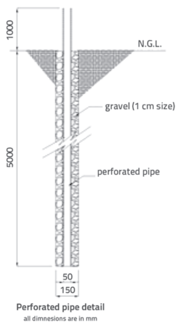
Figure 4. Well point pipe details (N.G.L - Natural Ground Level)
