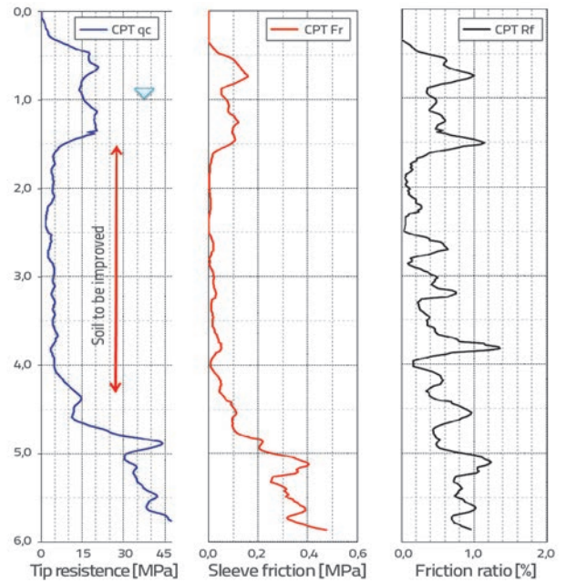
Figure 3. CPT representing soil profile
