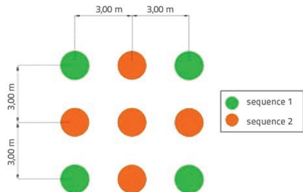
Figure 5. Compaction points layout
