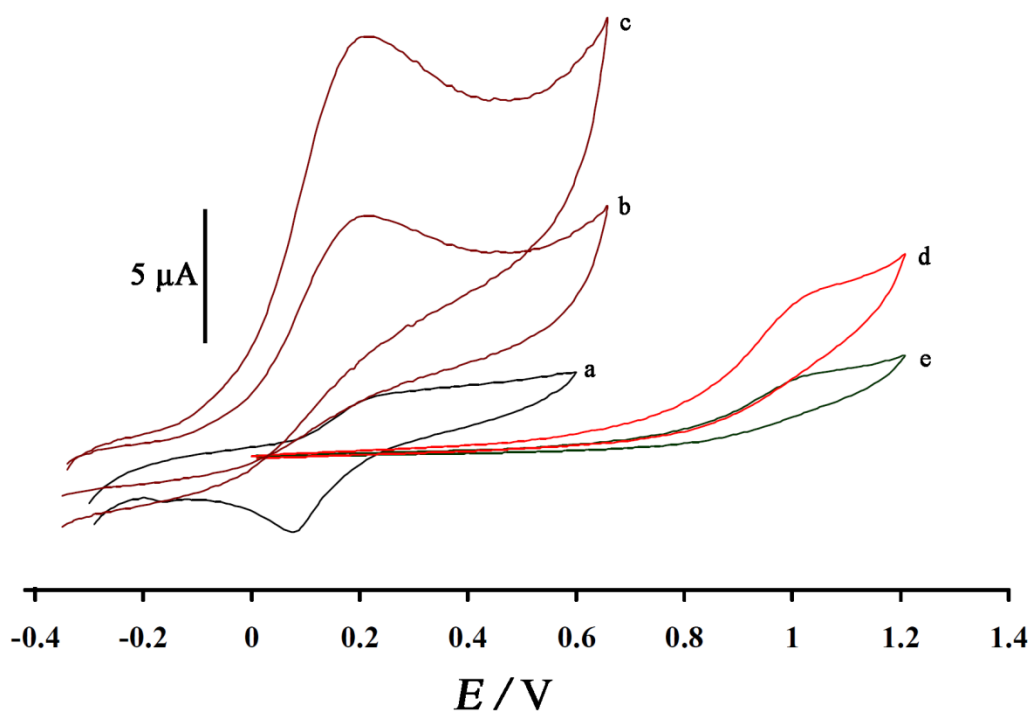
Figure 2. Cyclic voltammograms of (a) the buffer solution at DED/NiO/NPs/CPE; (b) 400 \mu\text{M} HX at DED/CPE; (c) 400 \mu\text{M} HX at DED/NiO/NPs/CPE; (d) 400. \mu\text{M} HX at NiO/NPs/CPE; (e) 400 \mu\text{M} HX at CPE. Conditions: 0.1 mol L -1 PBS (pH 8.0), scan rate of 20 mV s -1 .
