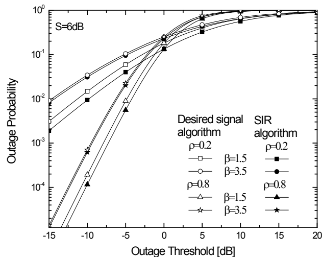
Figure 2 The comparison of system outage probability when desired signal algorithm and SIR based algorithm are employed for different values of correlation coefficient and fading parameter
