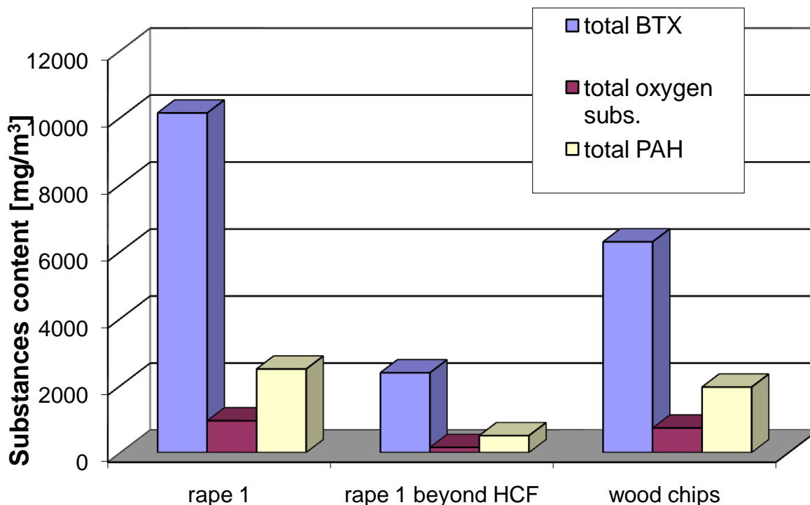
Figure 4. Tar compound content sampled before and beyond HCF during gasification of rape. To compare is there shown content of tar in gas from gasification wood chips
