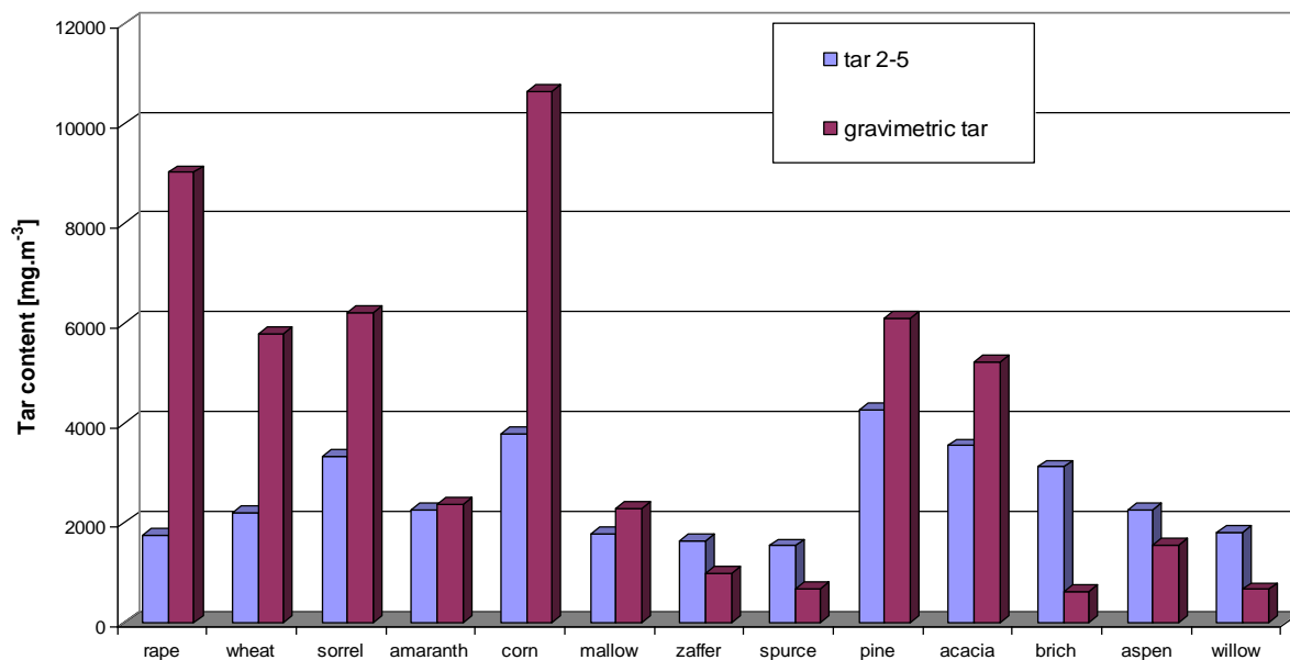
Figure 1. Comparison of tar content for stalk and woods [2]
