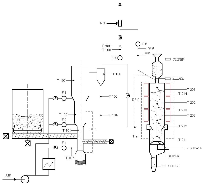
Figure 2. Scheme of experimental equipment BIOFLUID 100 Slika 2. Shema eksperimentalne opreme BIOFLUID 100
