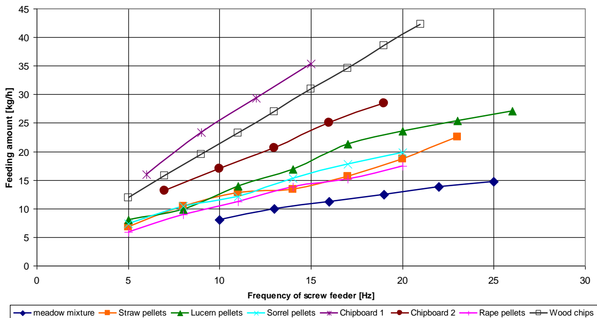
Figure 3. Results of testing of various fuels used in experimental gasification
